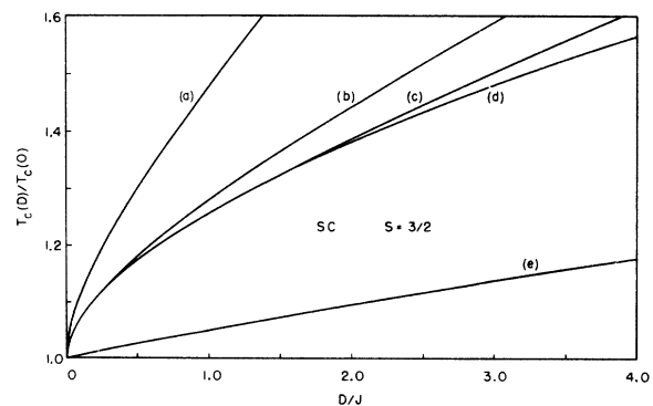
FIG. 7. The ratio T_c(D)/T_c(0) vs D/J for a sc spin S=3/2 ferromagnet. (a) Narath's results; (b) Anderson and Callen's results; (c) Lines's results; (d) results of this paper; (e) MFT results.
